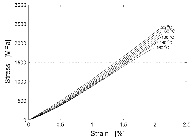
Fig. 2 Average stress versus strain curves using a mechanical strain gauge at all temperatures for Kevlar 49
