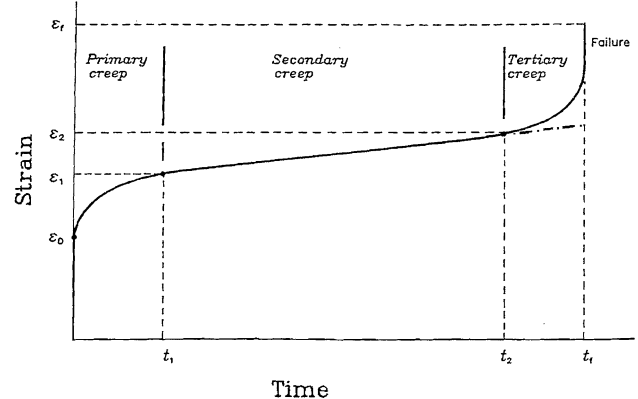
Fig. 14 Schematic creep curve [1]
